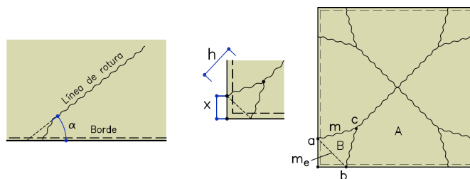
Fig. 1. Breaking lines on an edge and in a corner
