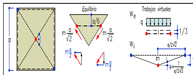
Fig. 3. Analysis of a square slab with hinged supports by the equilibrium method and by the virtual works method
