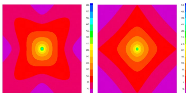
Fig. 9. Maximum moment view (left). Minimum moment (right)
