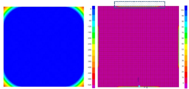
Fig. 5. Corner view. MEF
