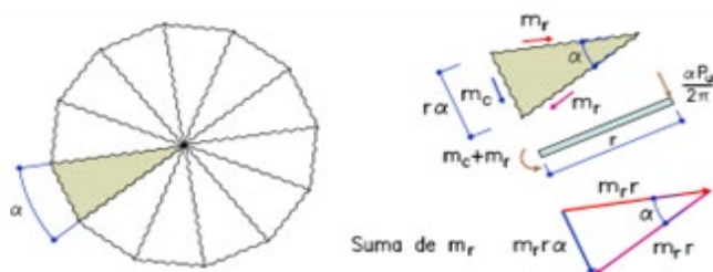
Fig. 2. Break lines of a slab subjected to a point load
