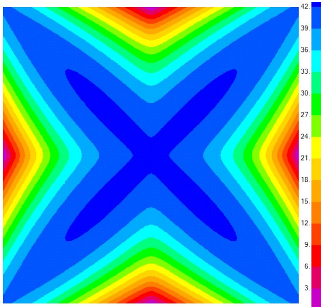
Fig. 4. Result with the finite element method (view)
