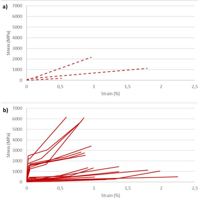
Fig. 8. Stress-strain idealized curves for FRCM systems for coated textile. a) Clevis b) Clamping
