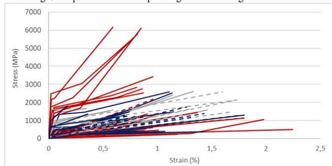
Fig. 6. Stress-strain idealized curves for FRCM systems. Blue lines are for dry textile, red for coated textile and grey lines for not specified. Dash lines are for clevis and continuous lines for clamping.
