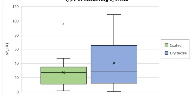
Fig. 17. Ratio ultimate load/control load ( \Delta P_u ) depending on the coating of the textile.
