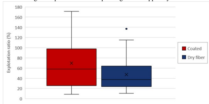
Fig. 5. Exploitation ratio depending on the coating of the textiles.
