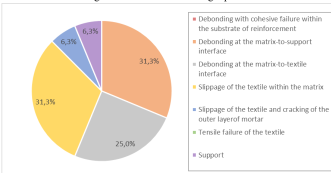
Fig. 4. Failure modes bending 5 points.
