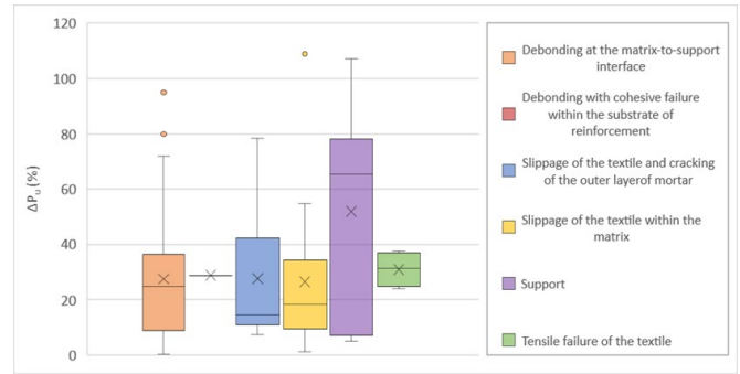
Fig. 15. Ratio ultimate load/control load ( \Delta P_u ) depending on failure mode.
