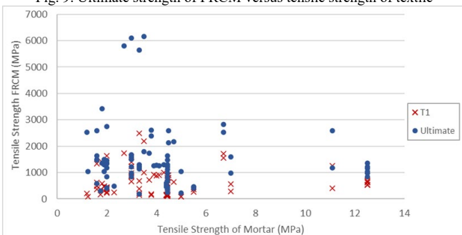
Fig. 10. Pre cracking and ultimate tensile strength of FRCM versus tensile strength of mortar
