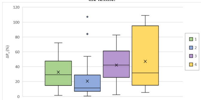
Fig. 18. Ratio ultimate load/control load ( \Delta P_u ) depending on the number of layers of textile.
