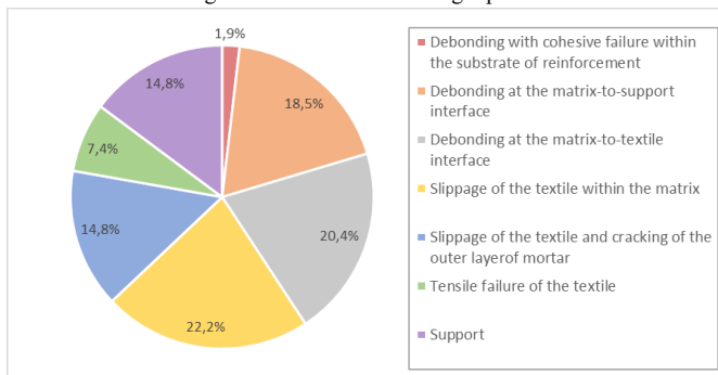
Fig. 3. Failure modes bending 4 points.
