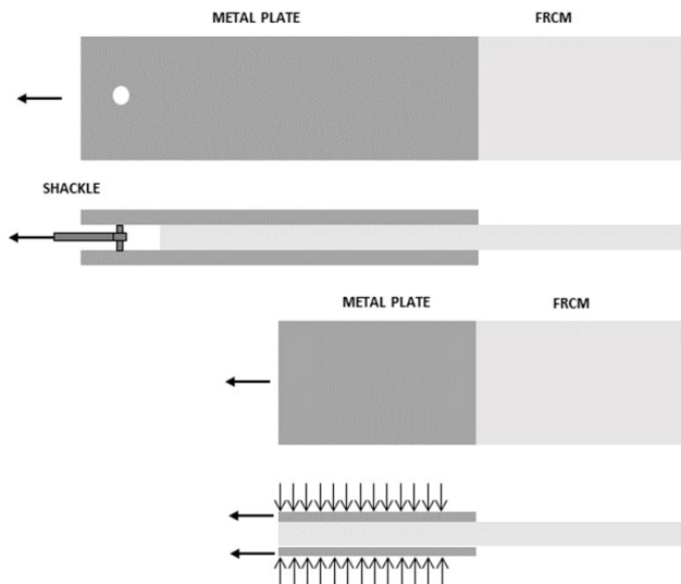
Fig. 2. Support systems: a) clevis b) clamping
