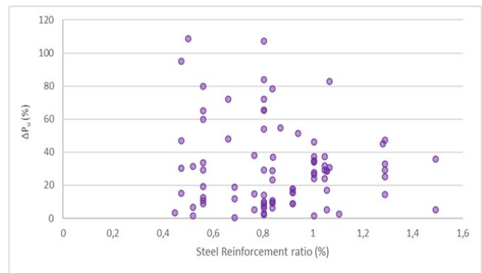
Fig. 20. Ratio ultimate load/control load ( \Delta P_u ) versus steel reinforcement ratio.
