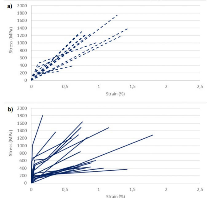
Fig. 7. Stress-strain idealized curves for FRCM systems for dry textile. a) Clevis b) Clamping.
