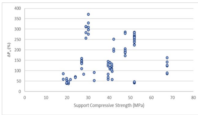
Fig. 19. Ratio ultimate load/control load ( \Delta P_u ) versus support compressive strength
