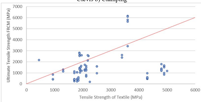
Fig. 9. Ultimate strength of FRCM versus tensile strength of textile
