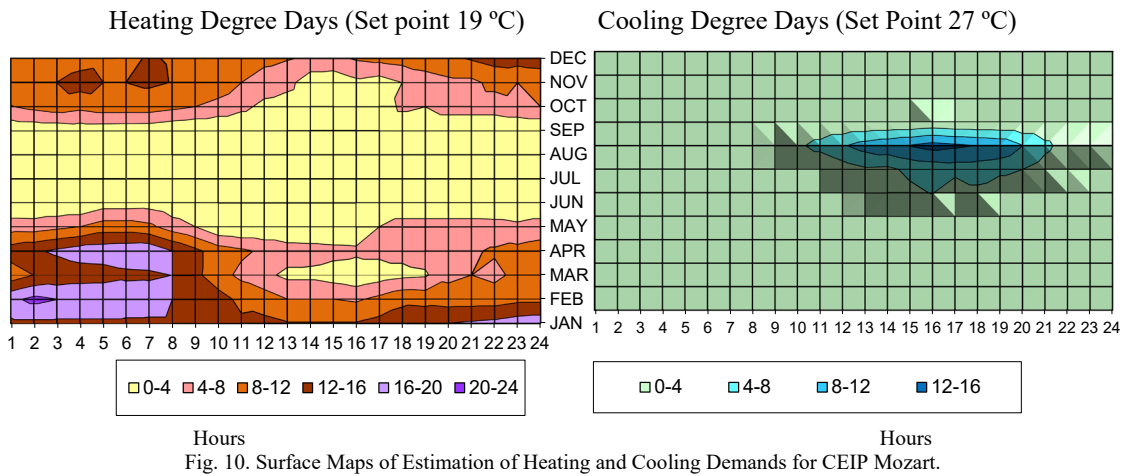
Fig. 10. Surface Maps of Estimation of Heating and Cooling Demands for CEIP Mozart.
