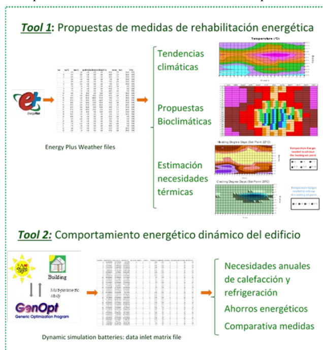
Fig. 5. Operating diagram of the energy rehabilitation toolkit developed within the framework of the project.
