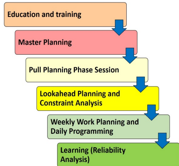
Fig. 1. Research methodology.
